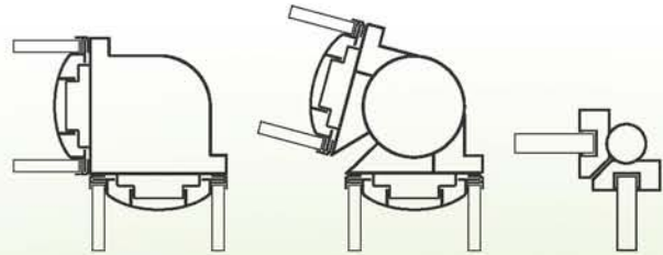
Corner Joint
