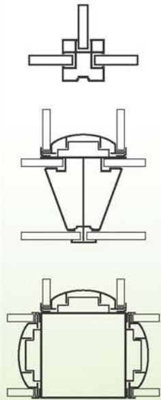
3-Ways Joint
